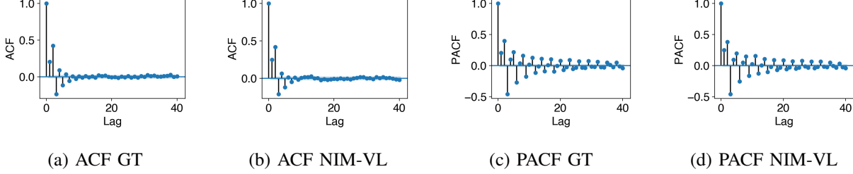
Figure 5: ACF and PACF for ARMA(3,3) process.
