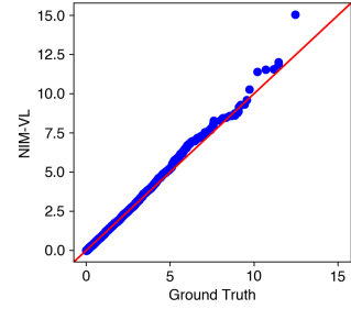
Figure 12: Q-Q plot for W_{60} distribution in a GI/G/1 queue.
