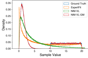
Figure 10: Empirical densities for Gamma-Uniform mixture.
